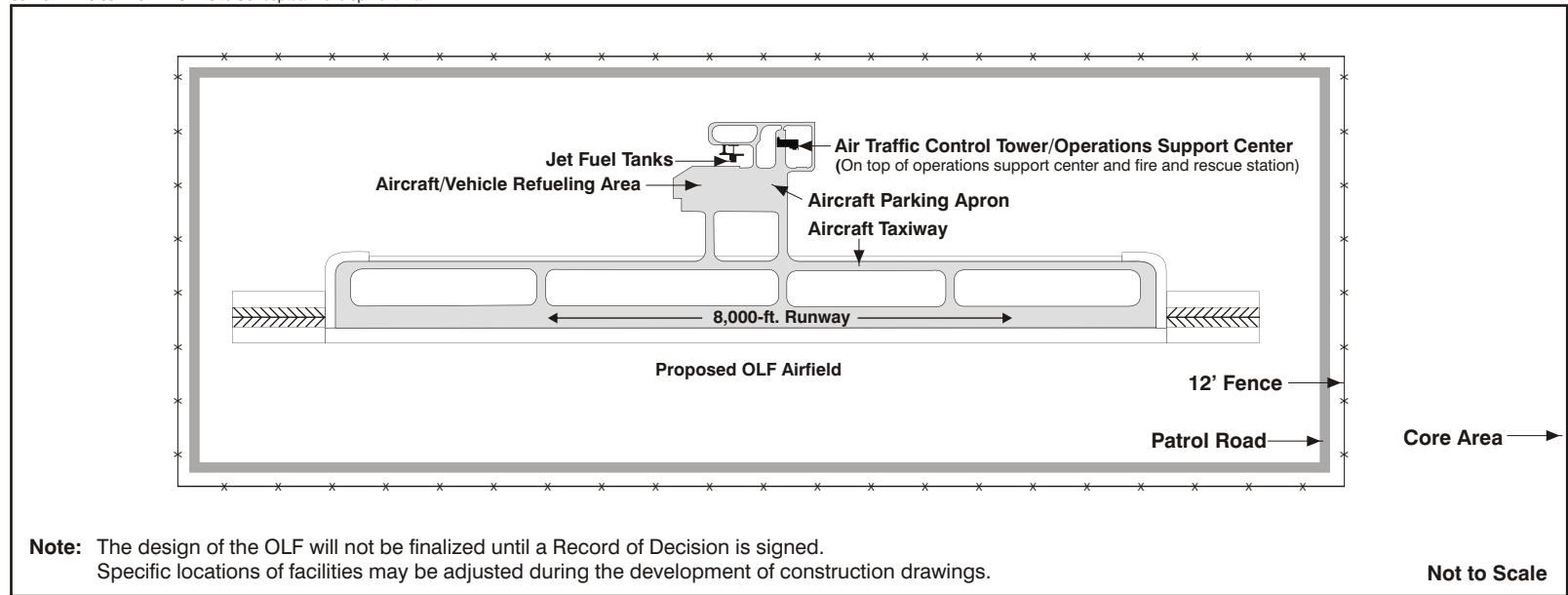
Figure A OLF Site Conceptual Development Plan
